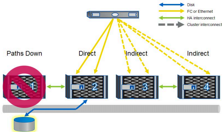
Figure 9) Paths during HA failover.
