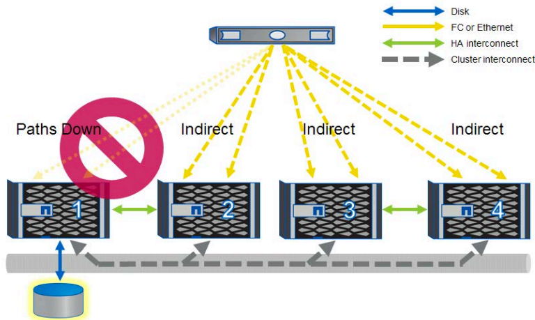
Figure 10) Paths during port or switch failure.
